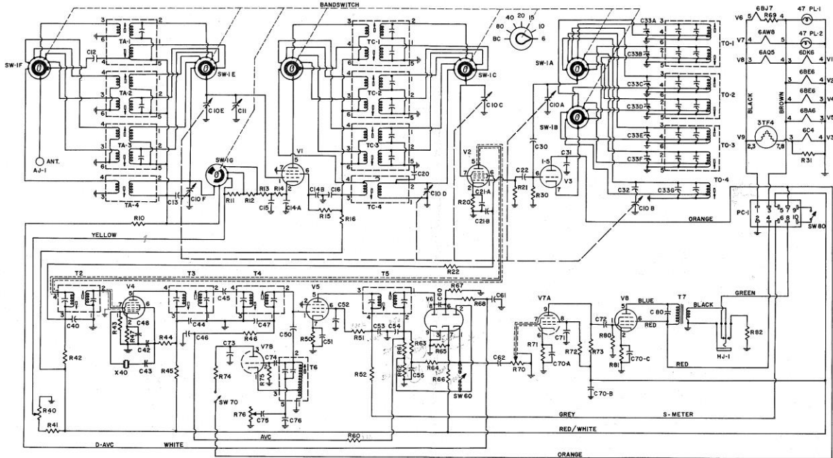
PMR-8 SCHEMATIC
